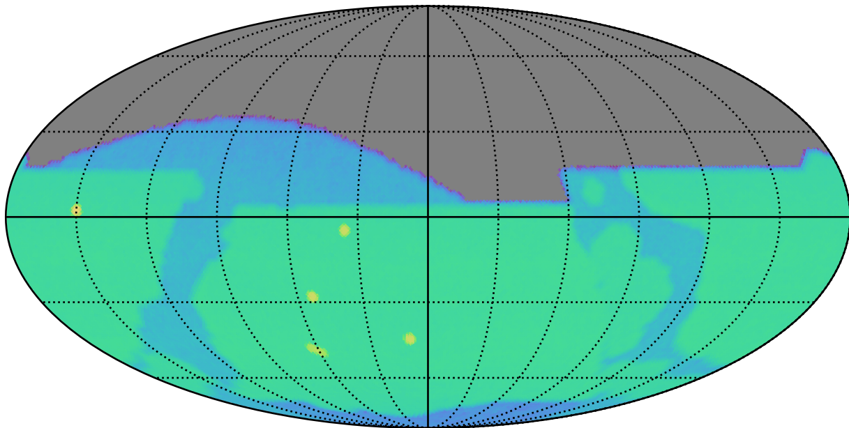
weather_cloudso8v3.4_10yrs z: SurfaceBrightLimit
