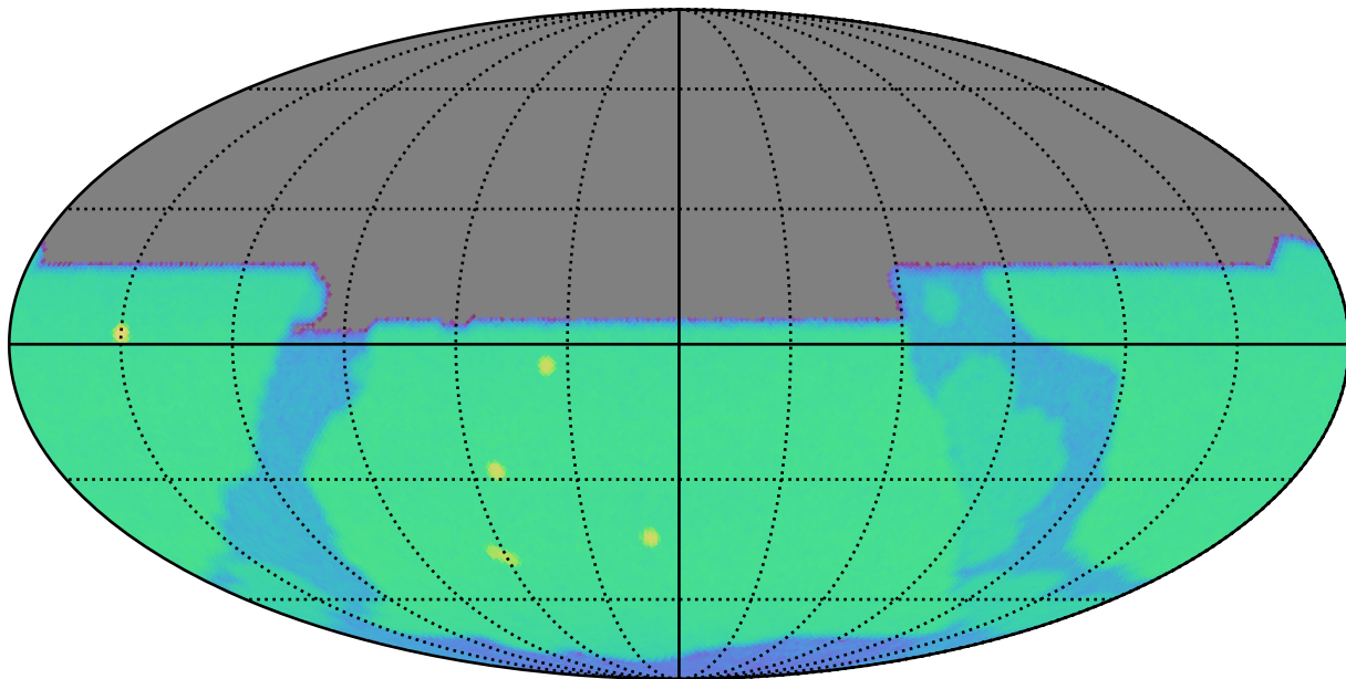
weather_cloudso8v3.4_10yrs y: SurfaceBrightLimit
