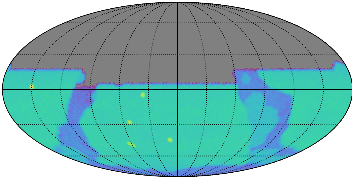
weather_cloudso8v3.4_10yrs u: SurfaceBrightLimit
