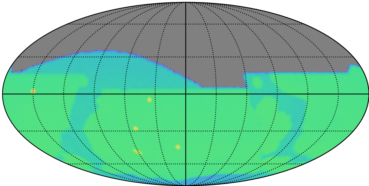
weather_cloudso8v3.4_10yrs r: SurfaceBrightLimit
