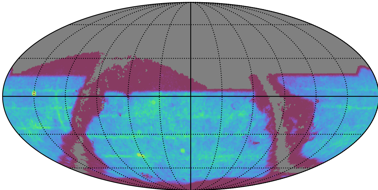
weather_cloudso8v3.4_10yrs : SNSLMetric
