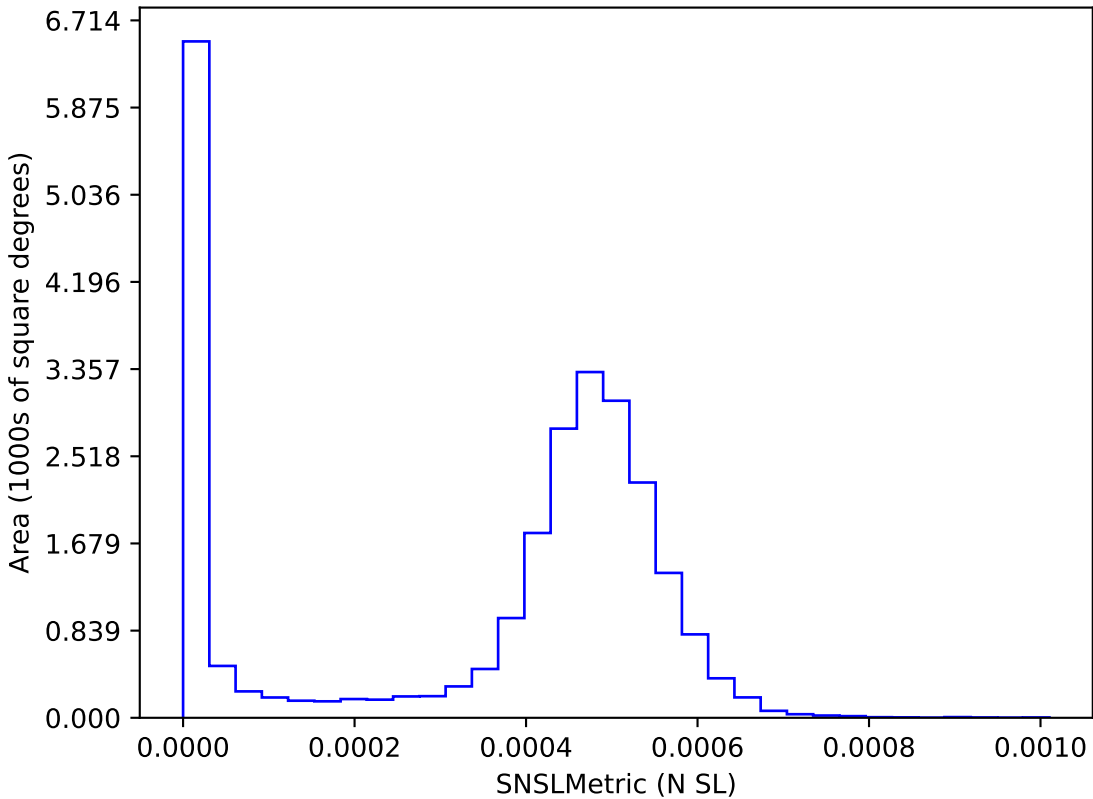
weather_cloudso8v3.4_10yrs : SNSLMetric
