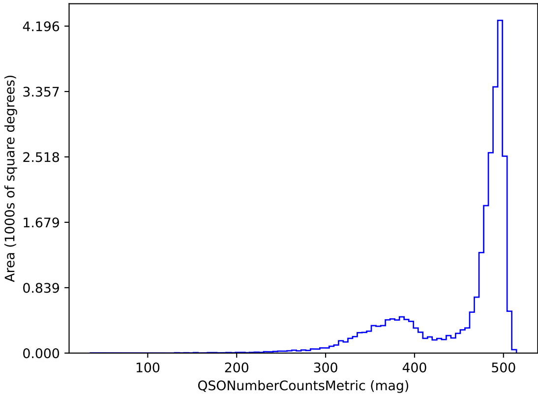
weather_cloudso8v3.4_10yrs z band and non-DD: QSONumberCountsMetric
