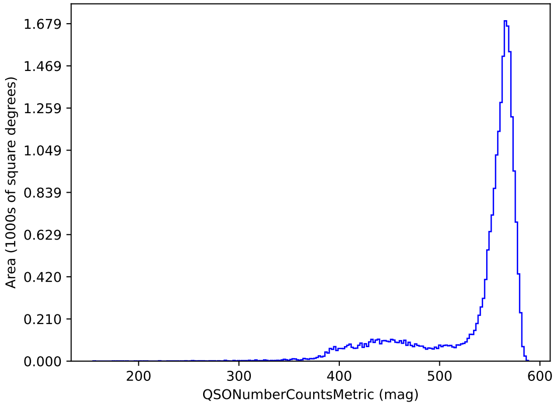
weather_cloudso8v3.4_10yrs y band and non-DD: QSONumberCountsMetric
