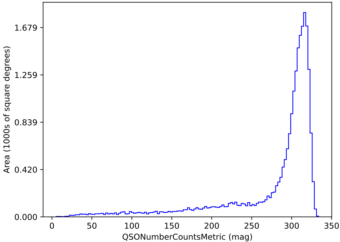
weather_cloudso8v3.4_10yrs u band and non-DD: QSONumberCountsMetric
