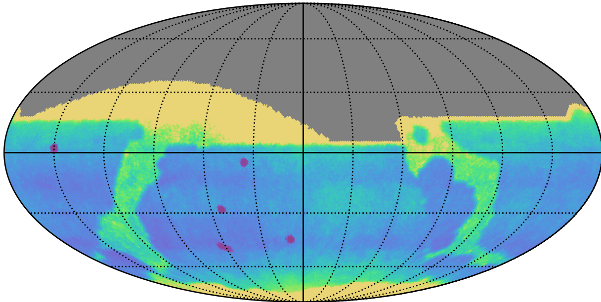
weather_cloudso8v3.4_10yrs : Proper Motion Uncert @ 24.0
