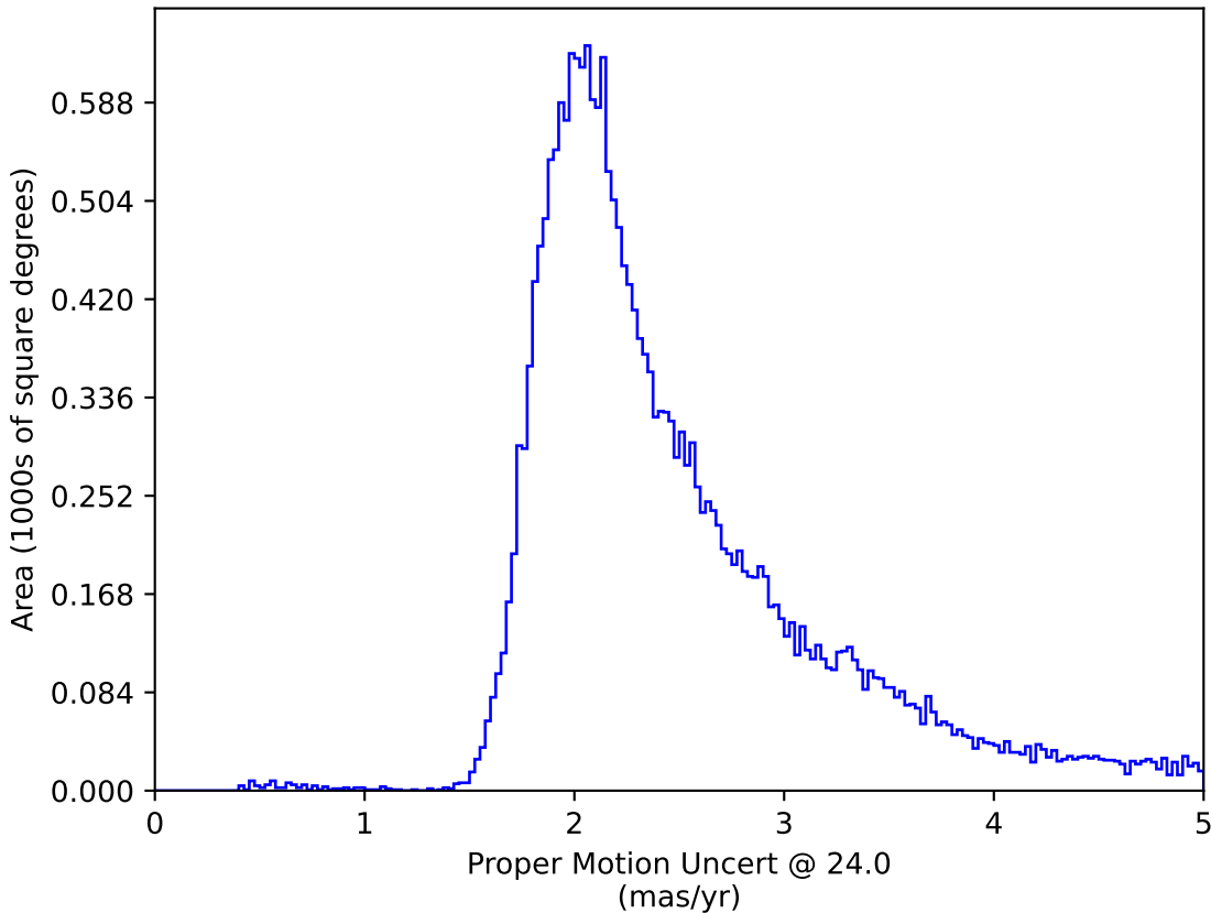
weather_cloudso8v3.4_10yrs : Proper Motion Uncert @ 24.0
