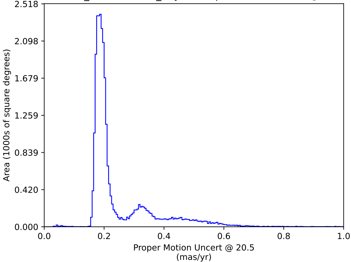
weather_cloudso8v3.4_10yrs : Proper Motion Uncert @ 20.5
