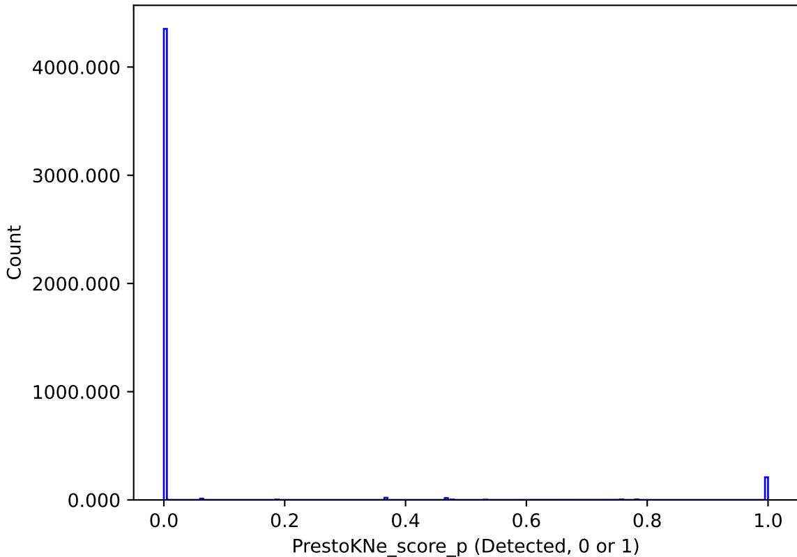
weather_cloudso8v3.4_10yrs : PrestoKNe_score_p
