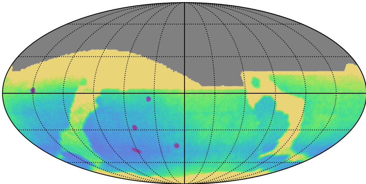
weather_cloudso8v3.4_10yrs : Parallax Uncert @ 24.0
