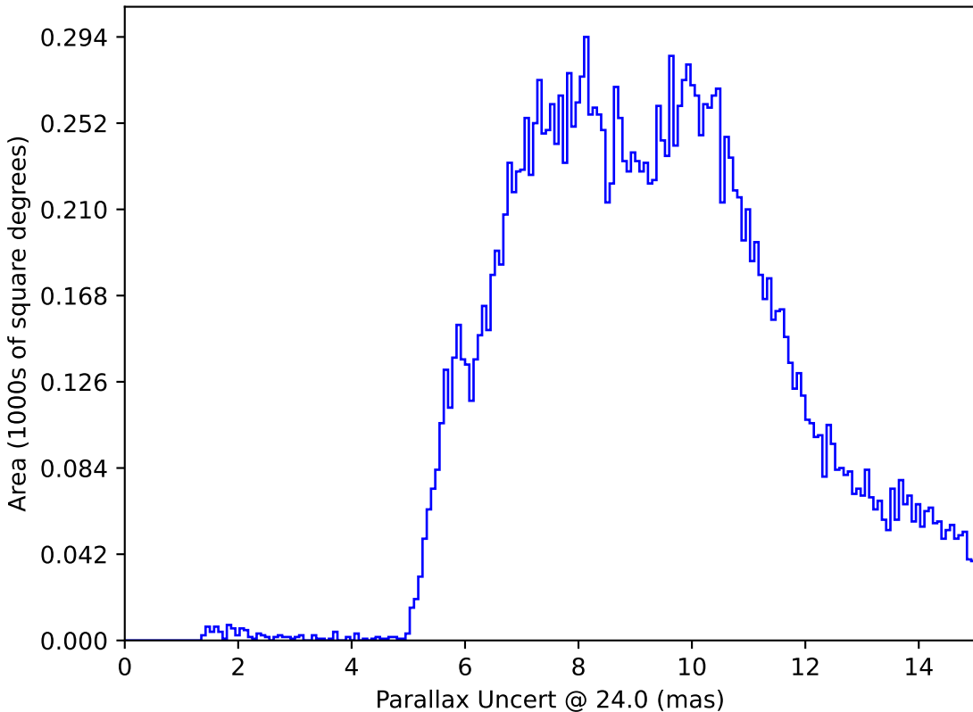
weather_cloudso8v3.4_10yrs : Parallax Uncert @ 24.0
