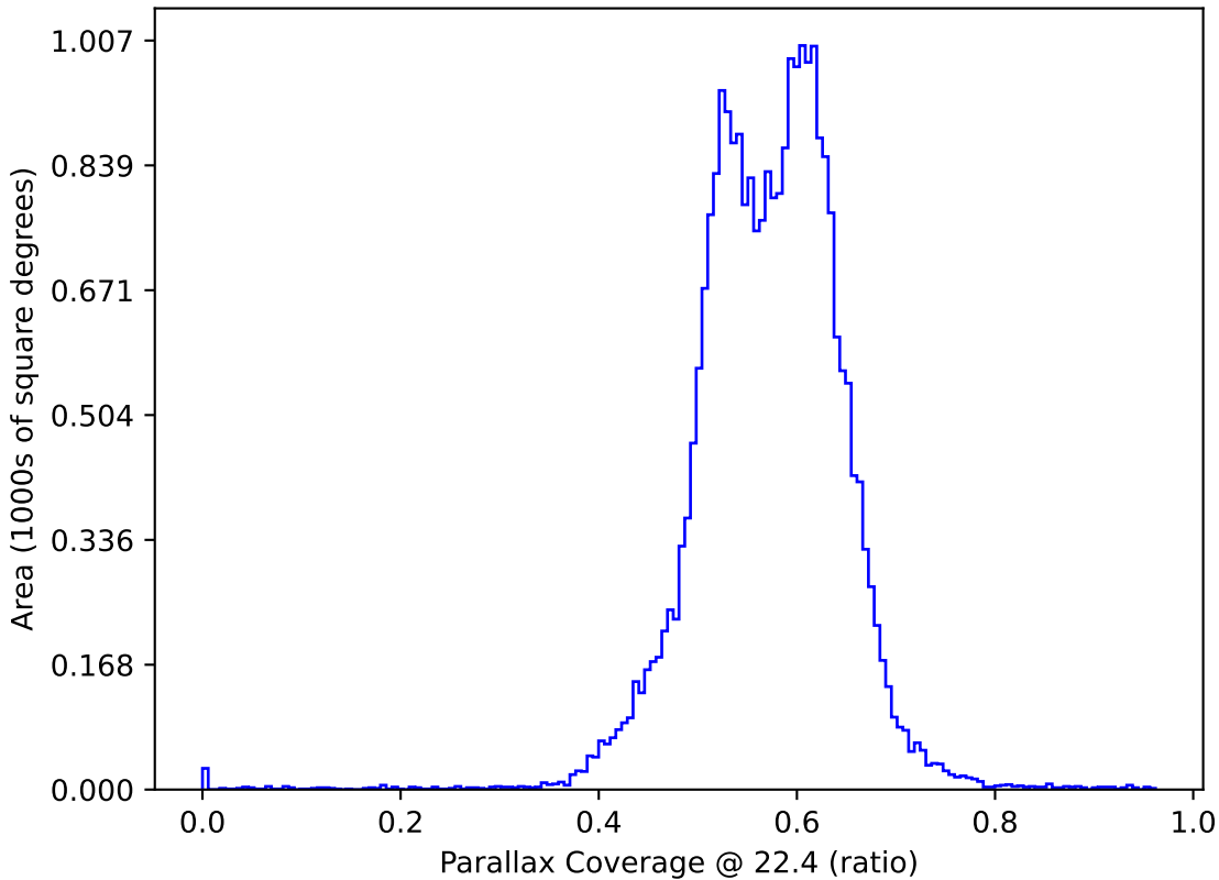
weather_cloudso8v3.4_10yrs : Parallax Coverage @ 22.4
