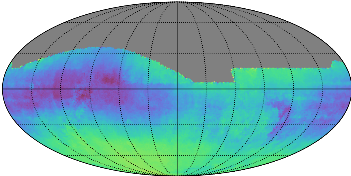
weather_cloudso8v3.4_10yrs : Parallax-DCR degeneracy @ 22.4
