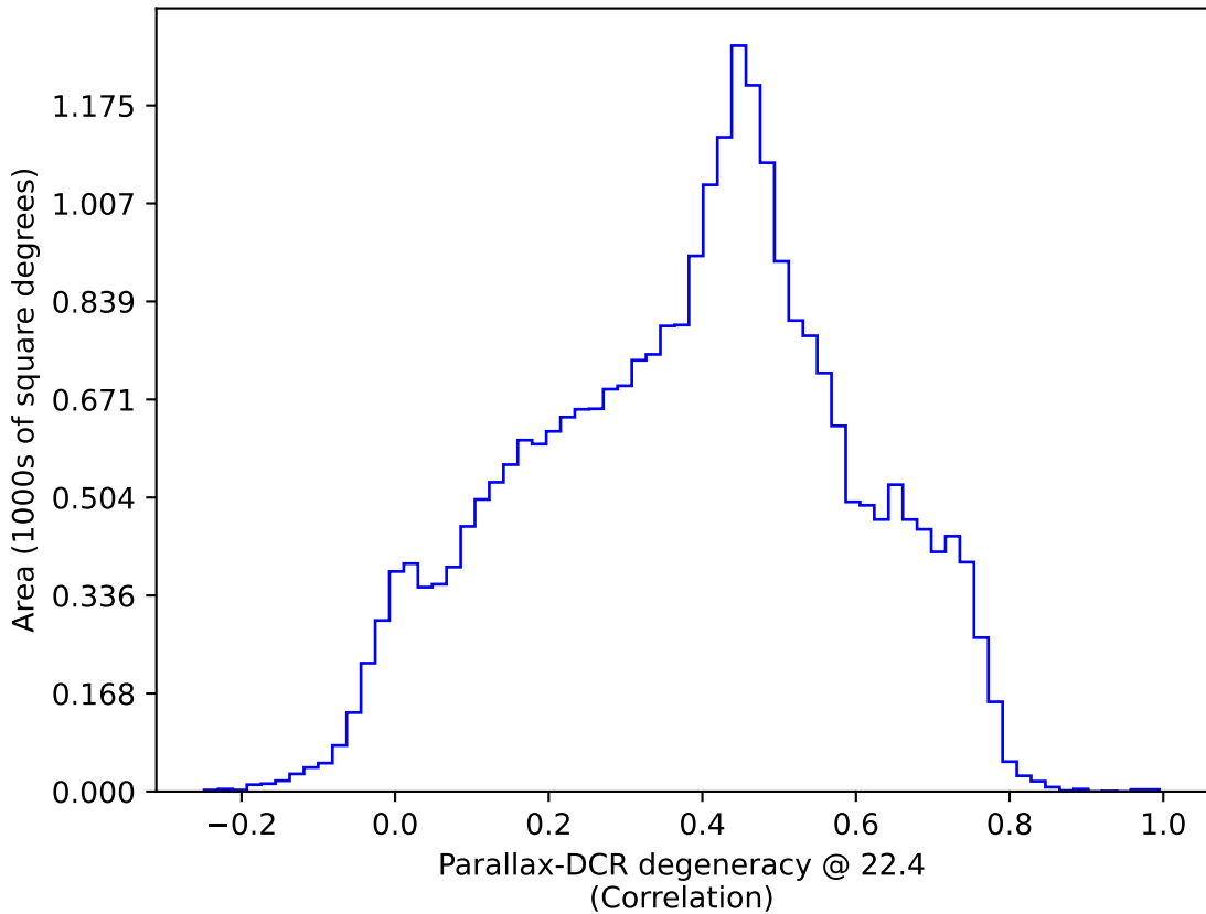
weather_cloudso8v3.4_10yrs : Parallax-DCR degeneracy @ 22.4
