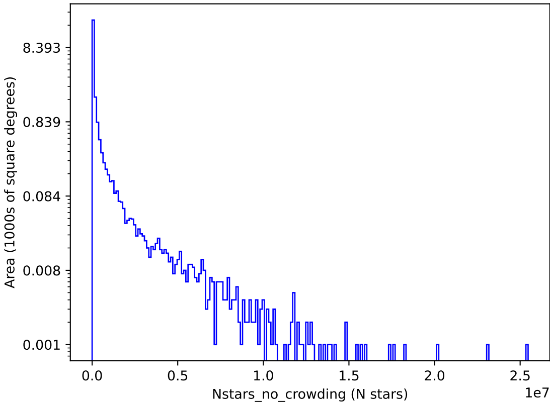
weather_cloudso8v3.4_10yrs y: Nstars_no_crowding
