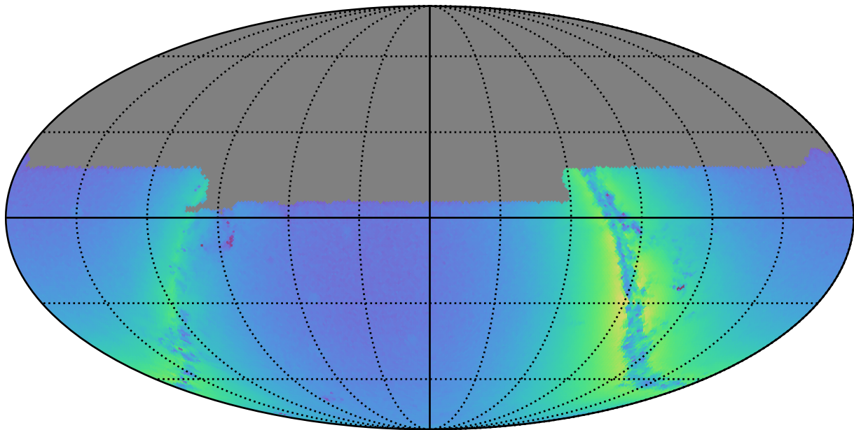
weather_cloudso8v3.4_10yrs u: Nstars_no_crowding
