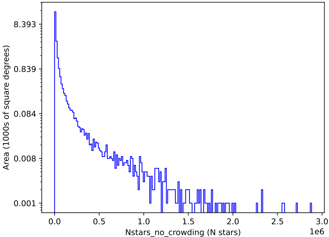
weather_cloudso8v3.4_10yrs u: Nstars_no_crowding
