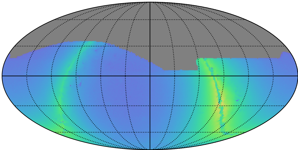
weather_cloudso8v3.4_10yrs r: Nstars_no_crowding
