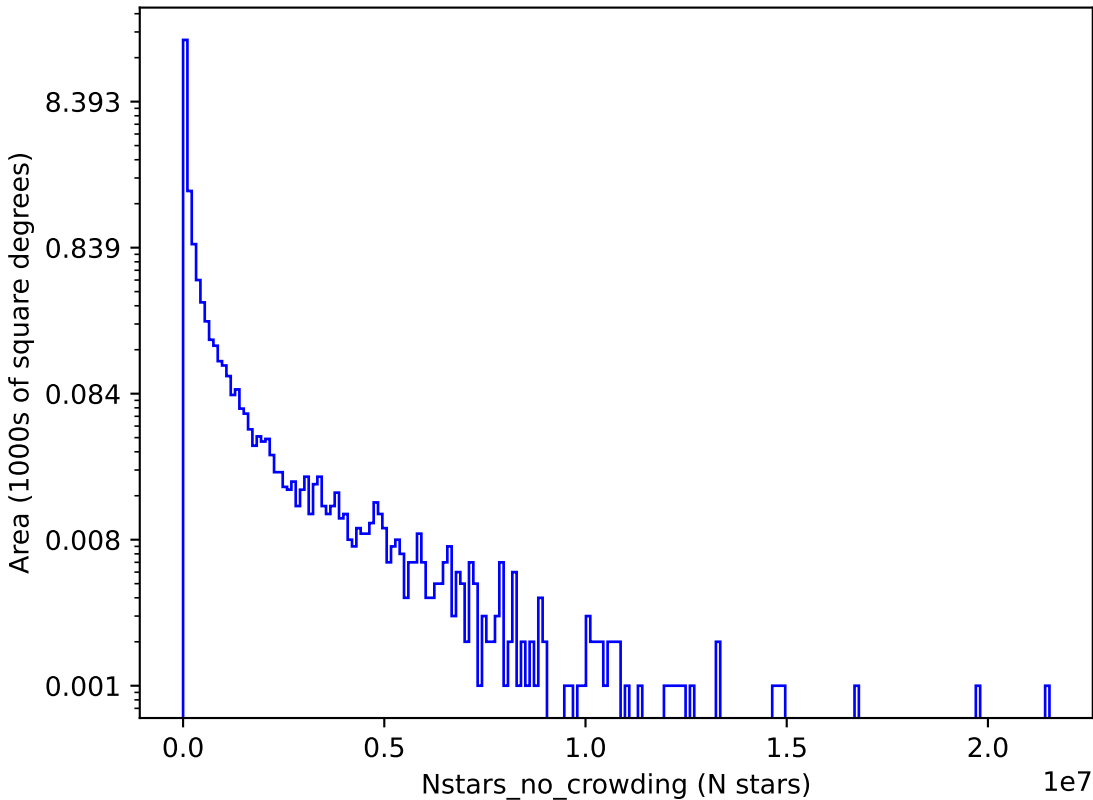
weather_cloudso8v3.4_10yrs r: Nstars_no_crowding
