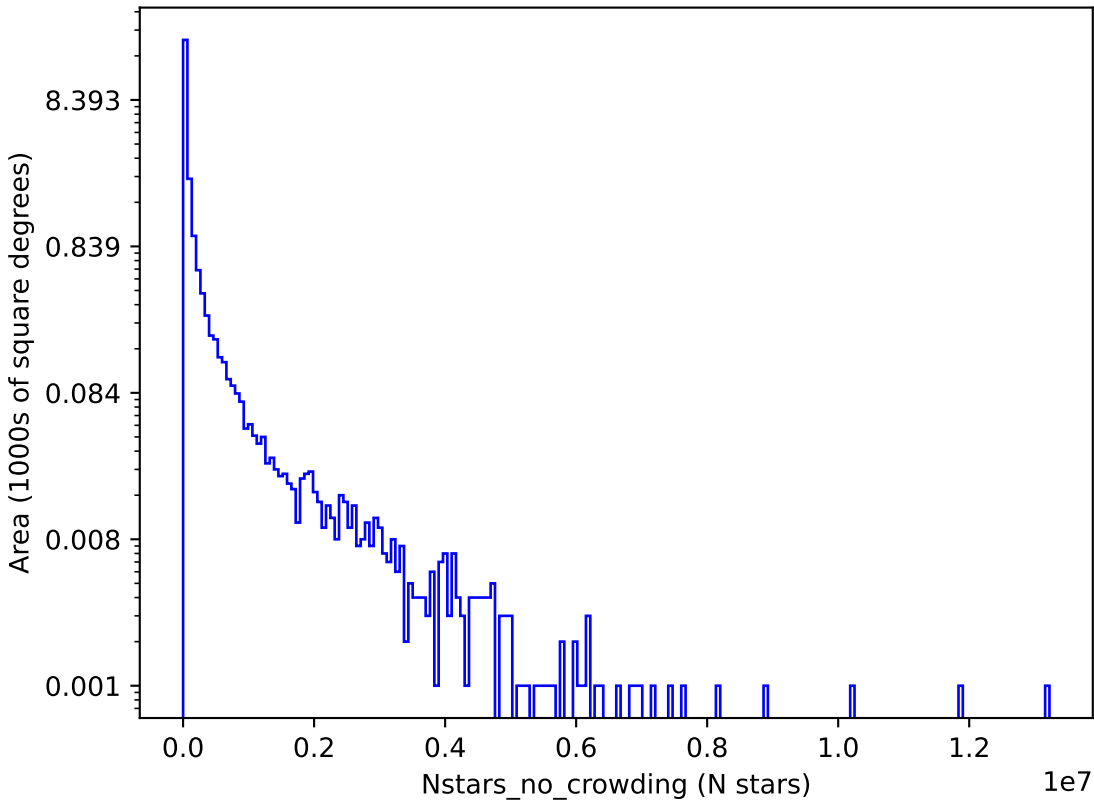
weather_cloudso8v3.4_10yrs g: Nstars_no_crowding
