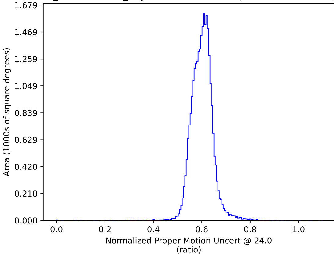
weather_cloudso8v3.4_10yrs : Normalized Proper Motion Uncert @ 24.0
