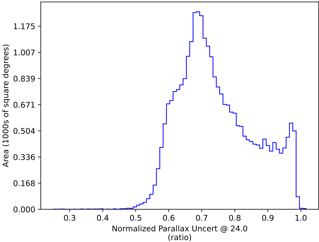
weather_cloudso8v3.4_10yrs : Normalized Parallax Uncert @ 24.0
