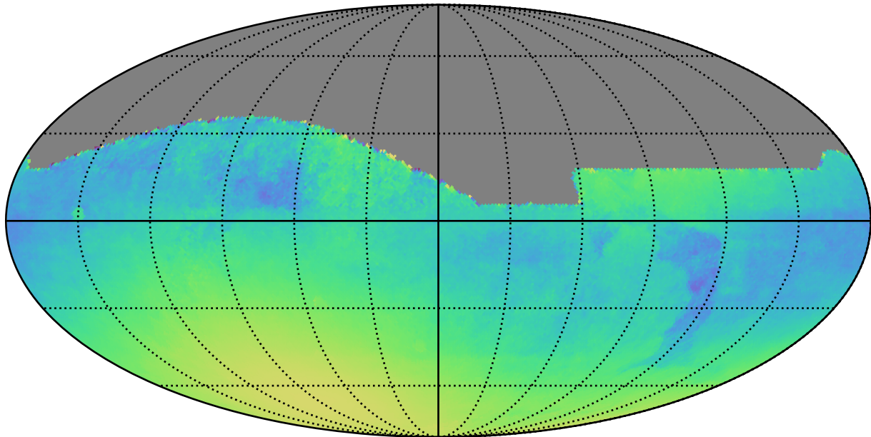
weather_cloudso8v3.4_10yrs : Normalized Parallax Uncert @ 22.4
