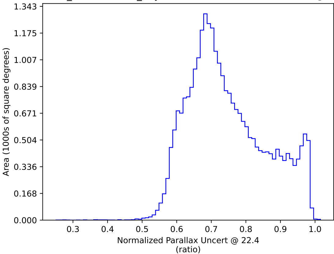
weather_cloudso8v3.4_10yrs : Normalized Parallax Uncert @ 22.4
