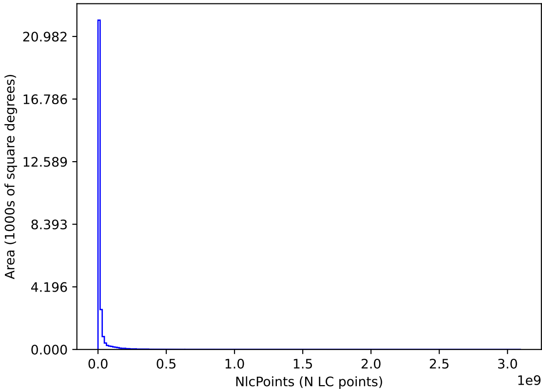
weather_cloudso8v3.4_10yrs : NlcPoints
