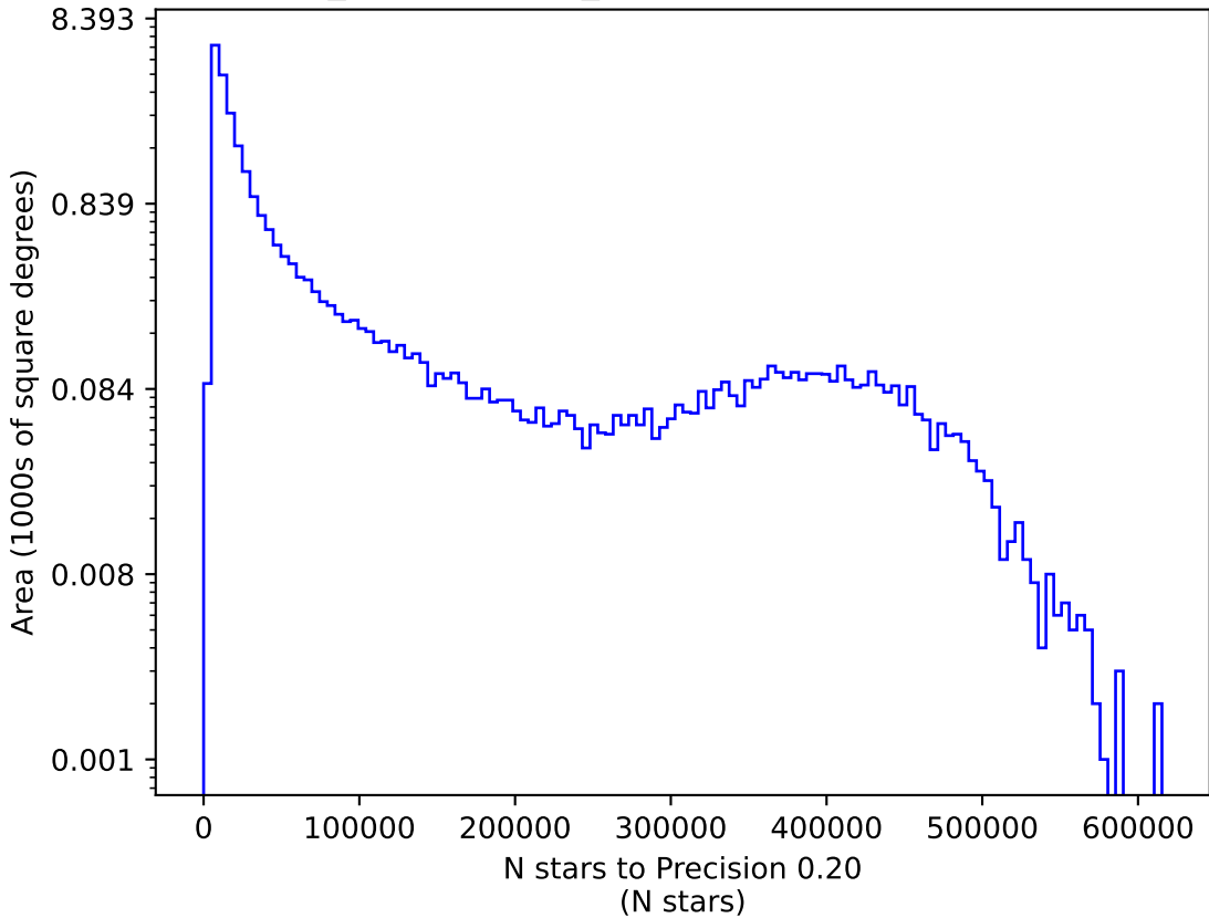
weather_cloudso8v3.4_10yrs z: N stars to Precision 0.20
