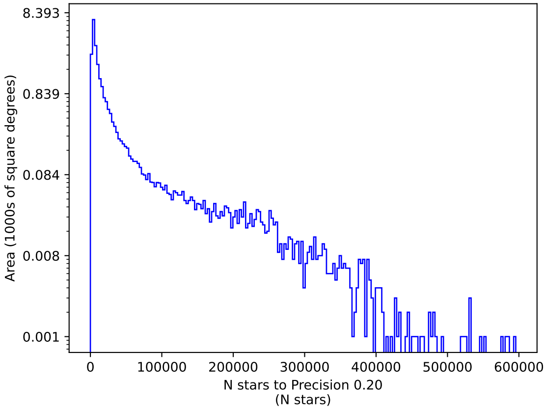
weather_cloudso8v3.4_10yrs u: N stars to Precision 0.20
