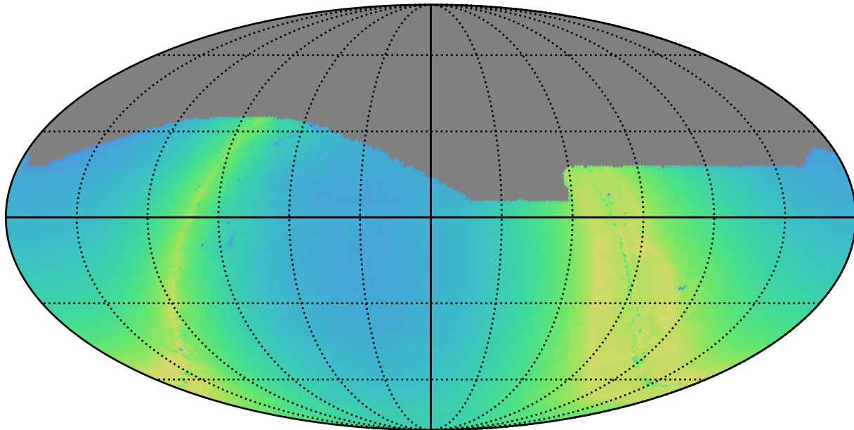
weather_cloudso8v3.4_10yrs r: N stars to Precision 0.20
