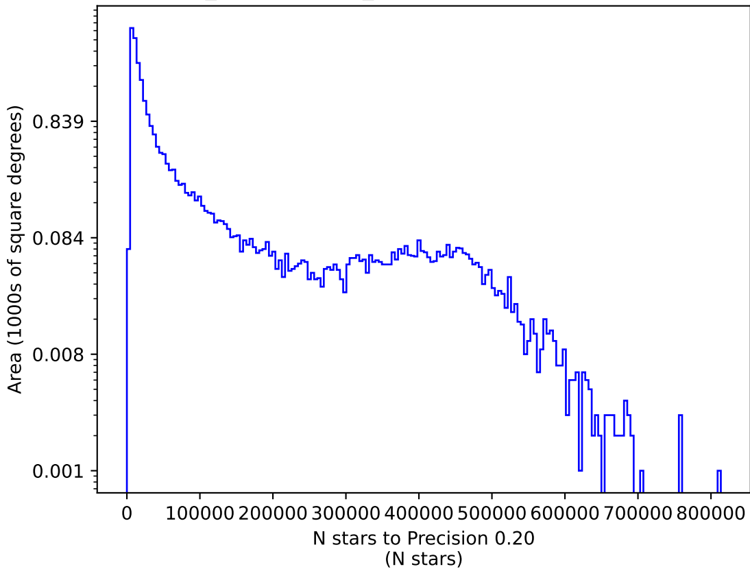
weather_cloudso8v3.4_10yrs r: N stars to Precision 0.20
