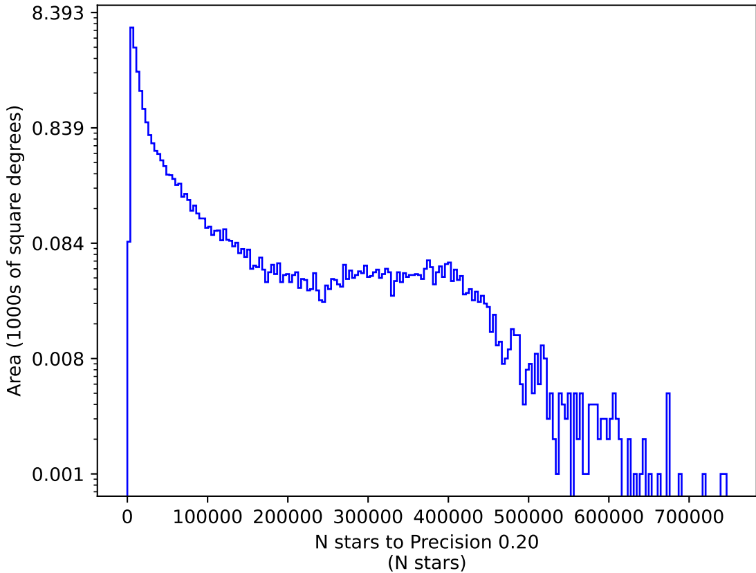
weather_cloudso8v3.4_10yrs g: N stars to Precision 0.20
