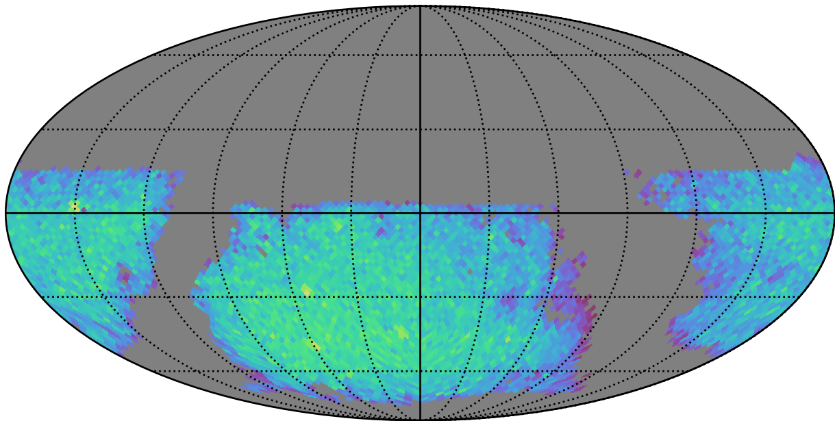
weather_cloudso8v3.4_10yrs gi: LVDwarfs
