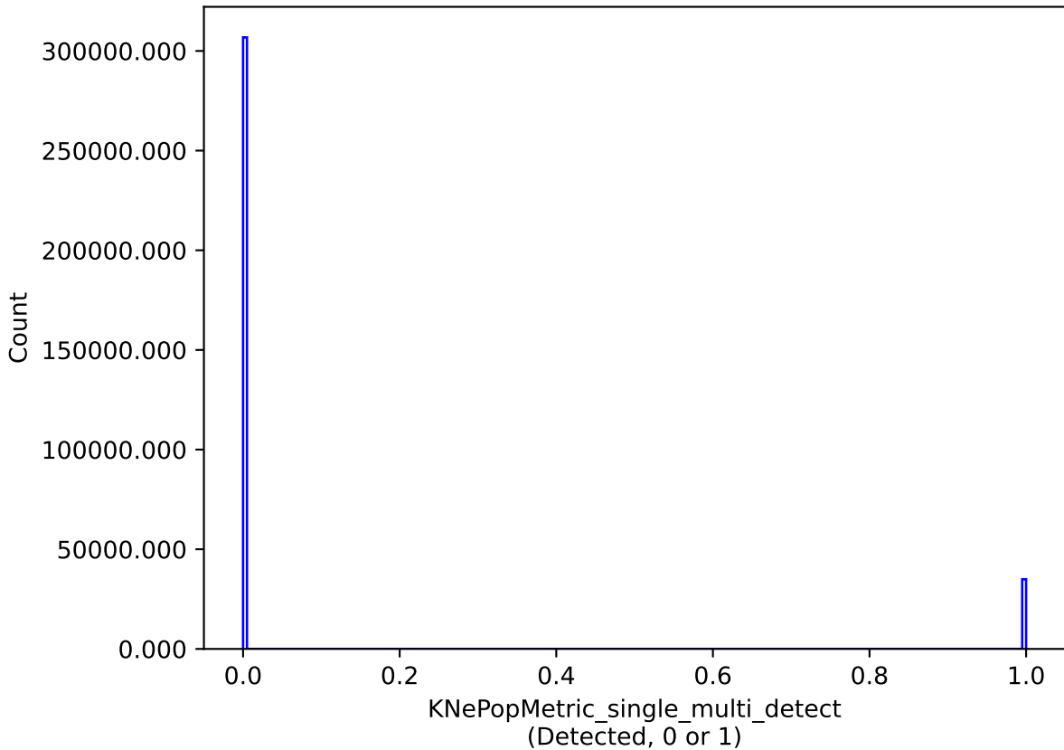
weather_cloudso8v3.4_10yrs single model: KNePopMetric_single_multi_detect
