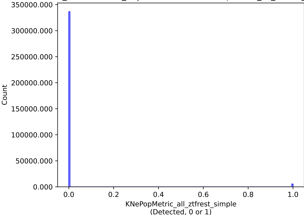
weather_cloudso8v3.4_10yrs all models: KNePopMetric_all_ztfrest_simple
