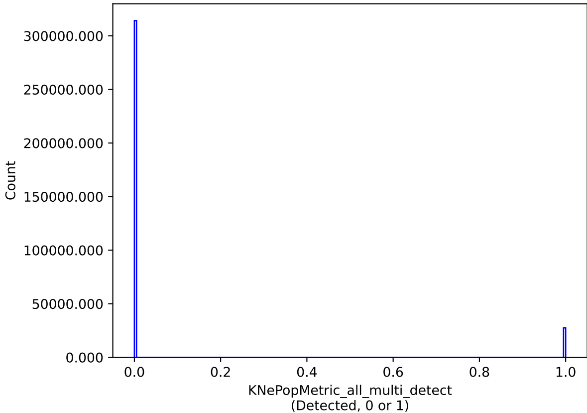
weather_cloudso8v3.4_10yrs all models: KNePopMetric_all_multi_detect
