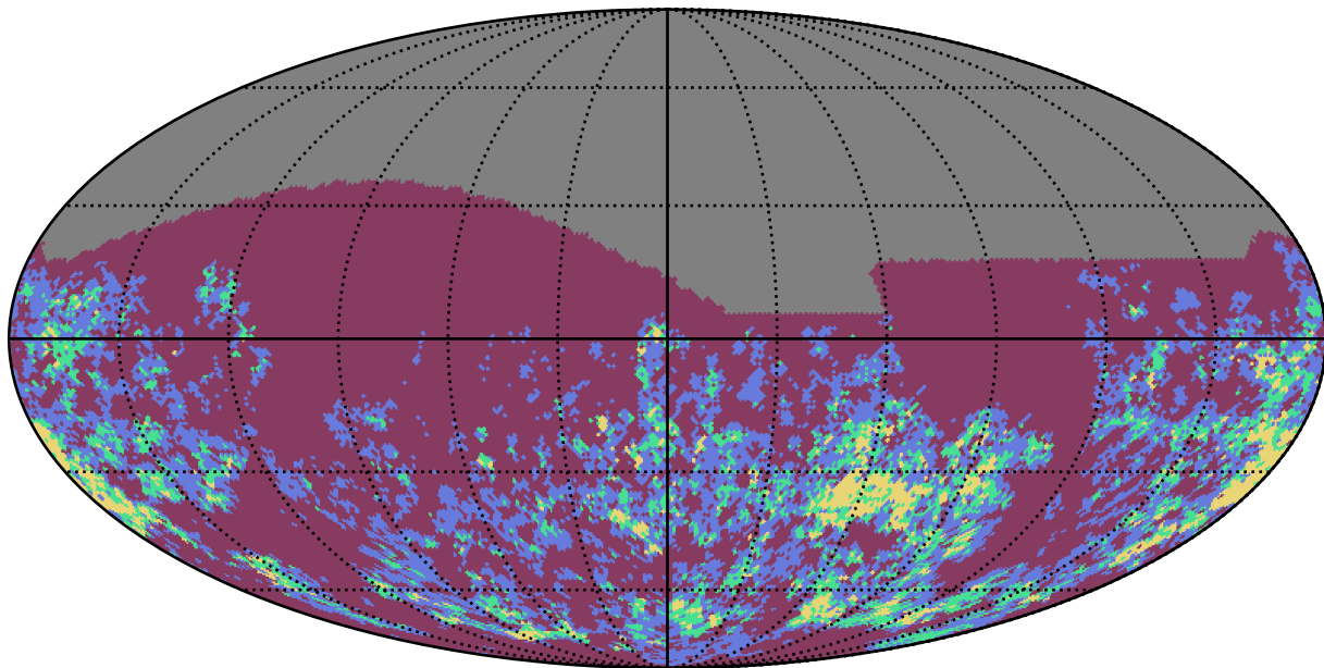
weather_cloudso8v3.4_10yrs z band: Gaps_7hr
