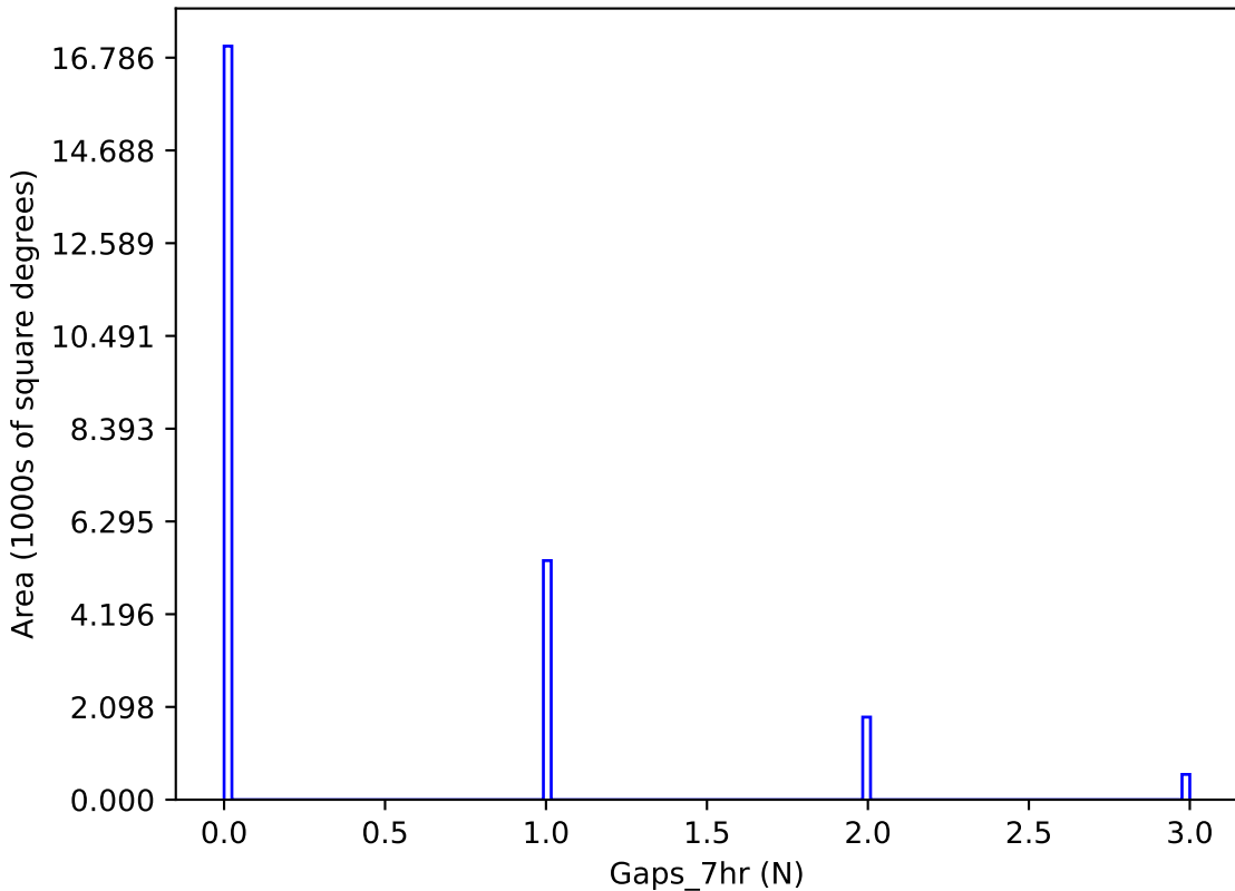
weather_cloudso8v3.4_10yrs y band: Gaps_7hr
