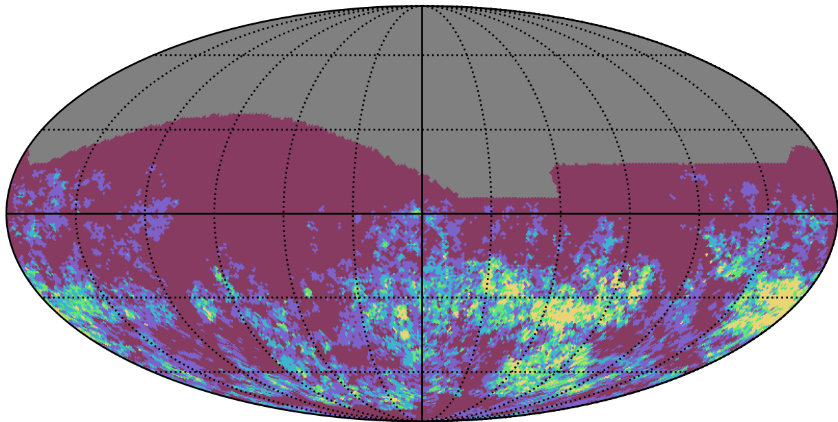
weather_cloudso8v3.4_10yrs i band: Gaps_7hr
