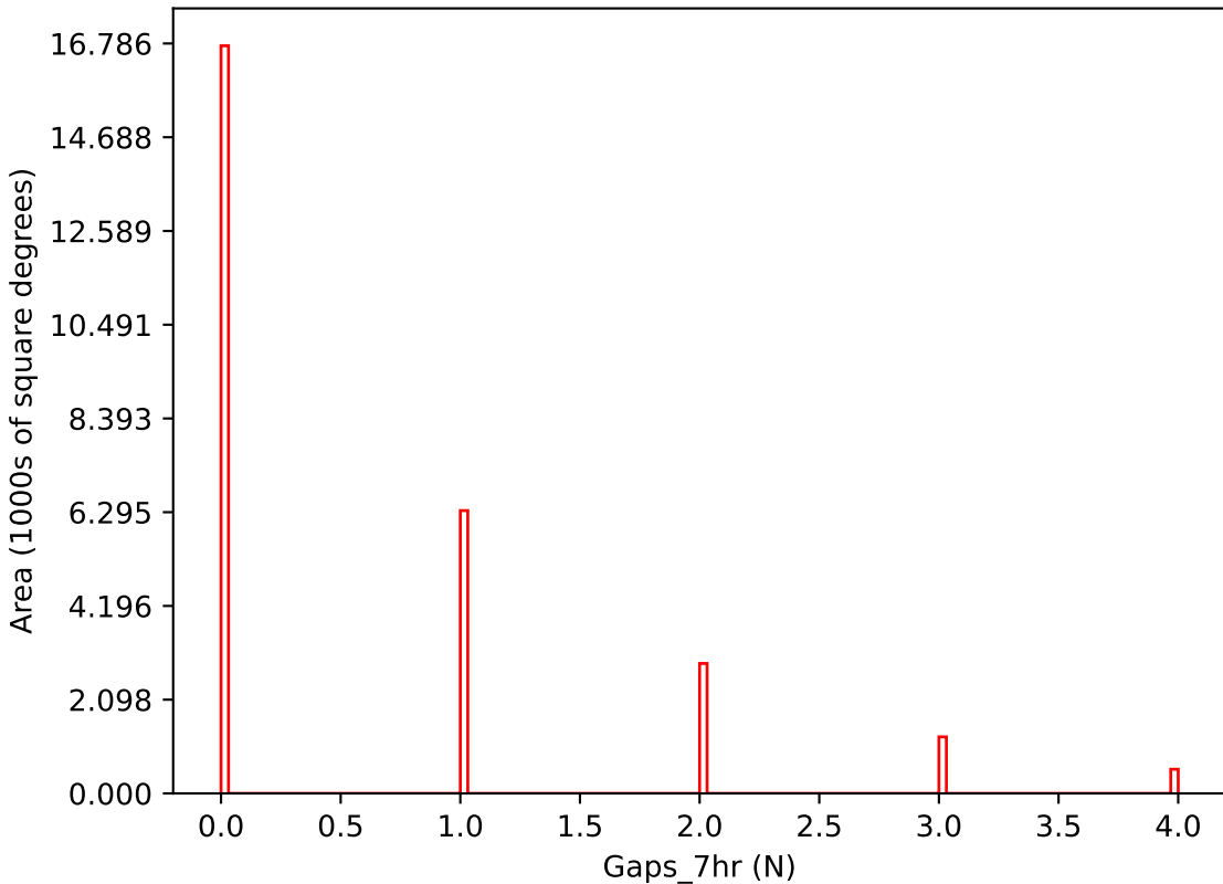
weather_cloudso8v3.4_10yrs i band: Gaps_7hr
