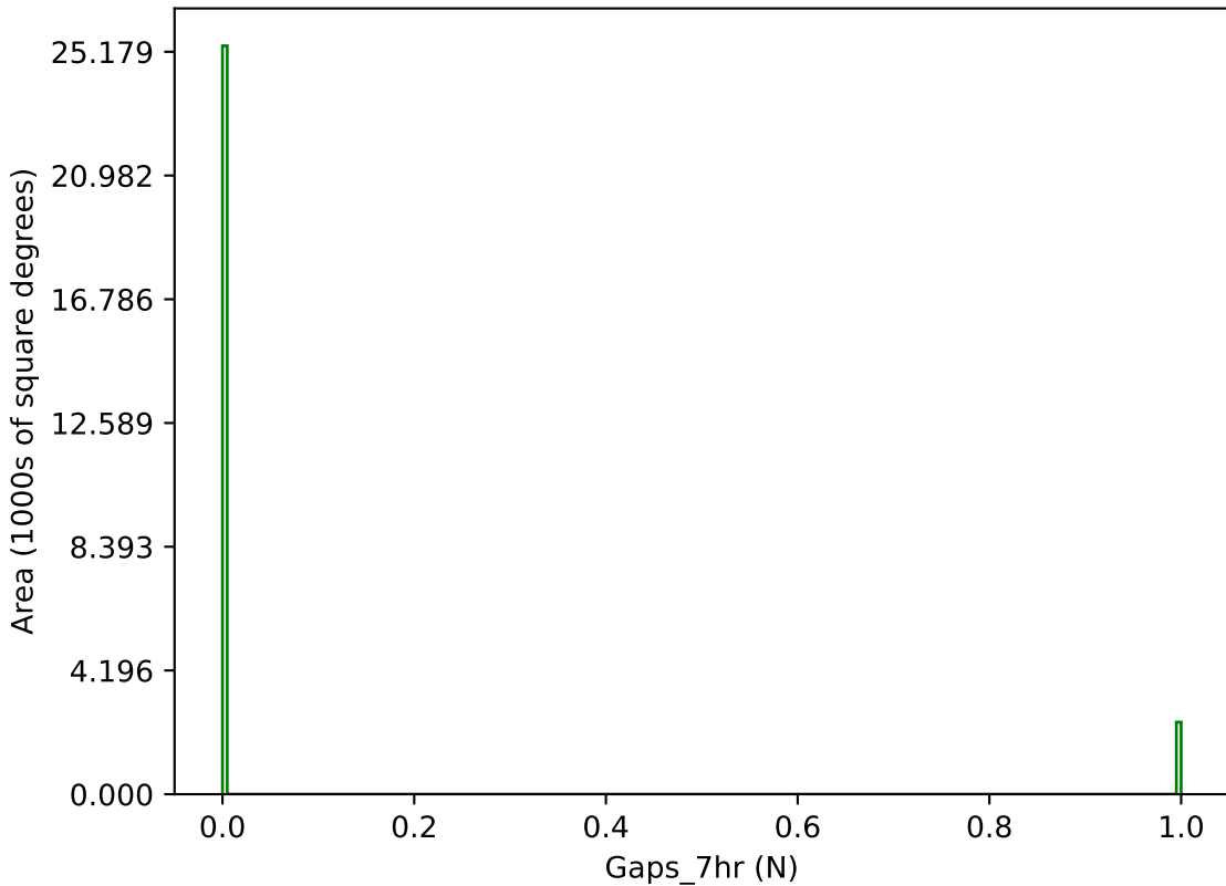
weather_cloudso8v3.4_10yrs g band: Gaps_7hr
