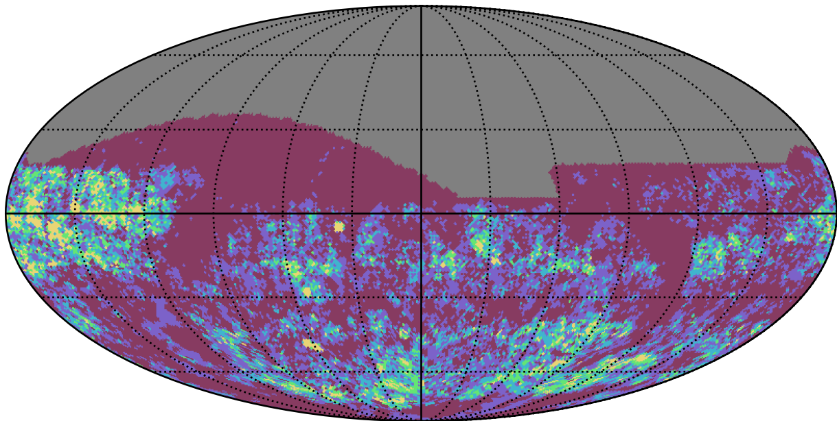
weather_cloudso8v3.4_10yrs z band: Gaps_3hr
