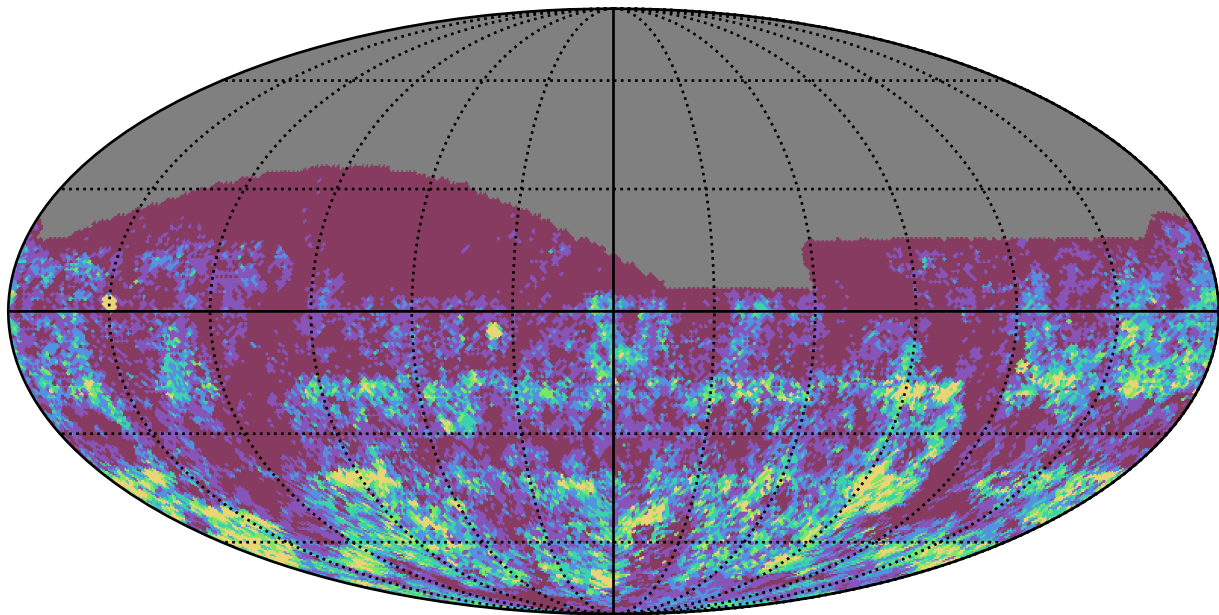
weather_cloudso8v3.4_10yrs r band: Gaps_3hr
