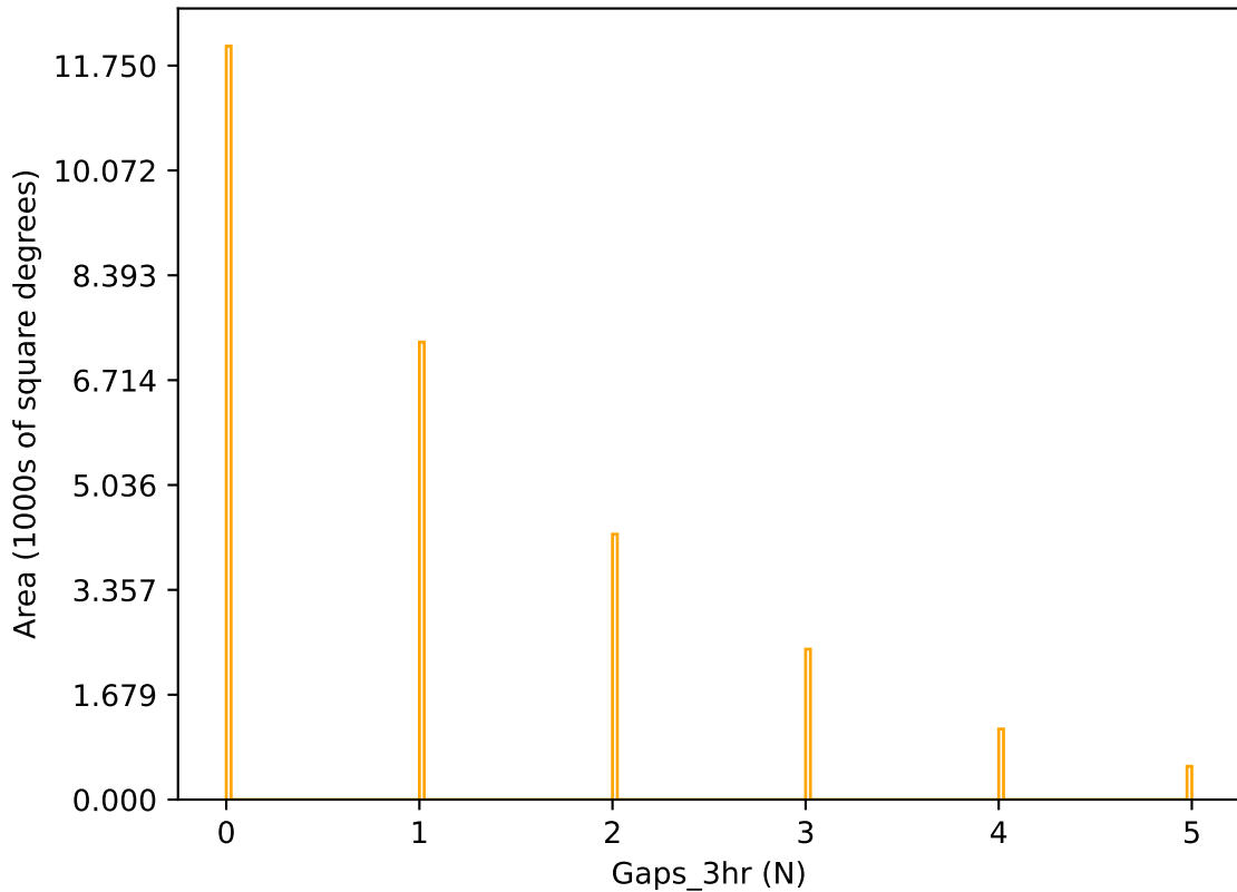
weather_cloudso8v3.4_10yrs r band: Gaps_3hr
