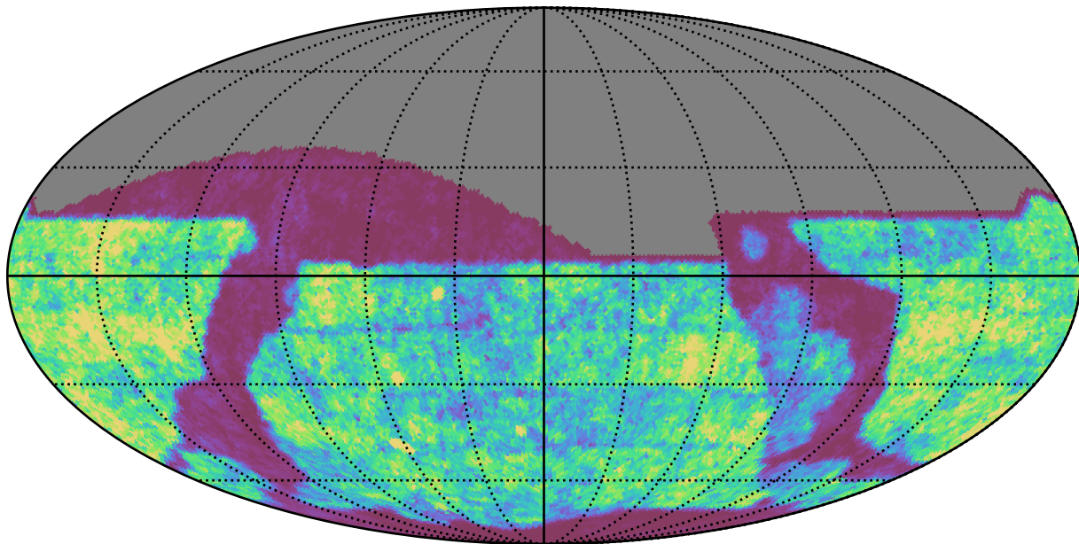
weather_cloudso8v3.4_10yrs z band: Gaps_24hr
