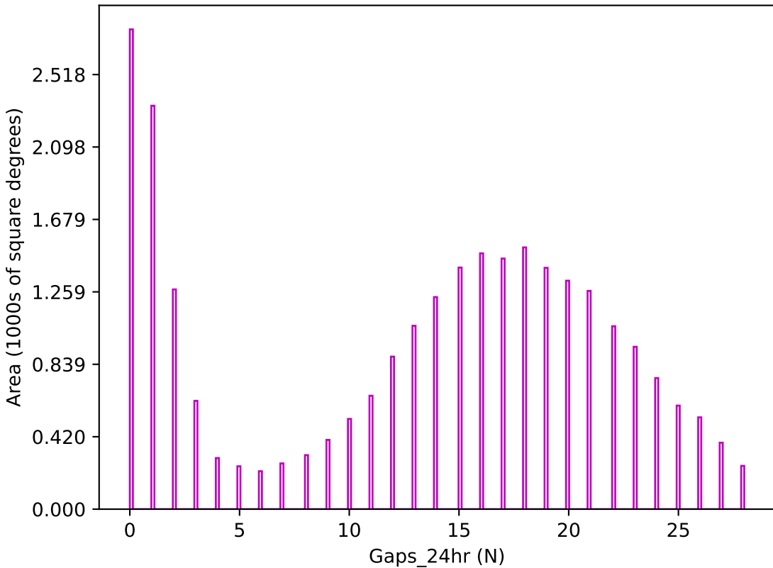
weather_cloudso8v3.4_10yrs z band: Gaps_24hr
