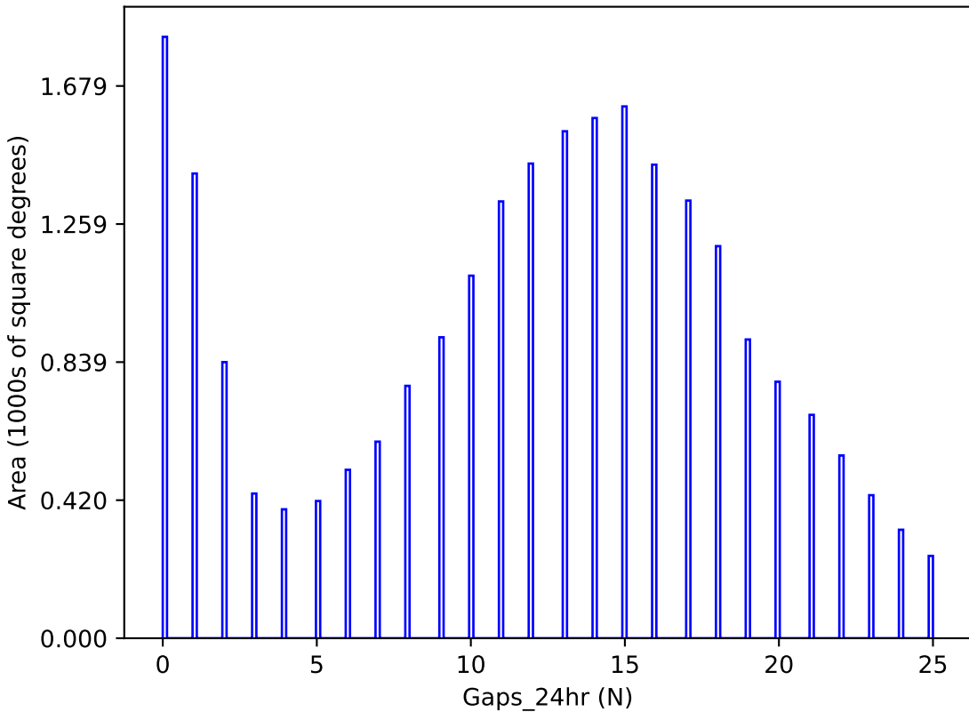
weather_cloudso8v3.4_10yrs y band: Gaps_24hr
