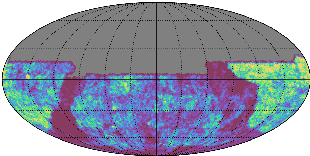
weather_cloudso8v3.4_10yrs u band: Gaps_24hr
